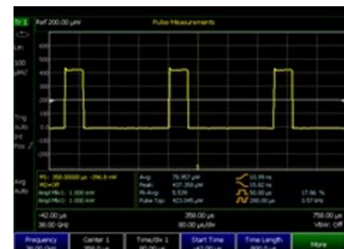
Use FieldFox to characterize pulses
