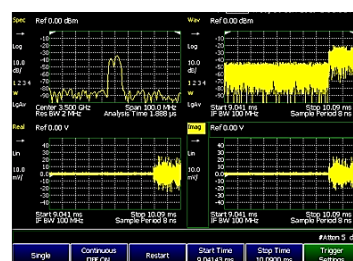
IQ data captured in FieldFox I/Q analyzer mode
