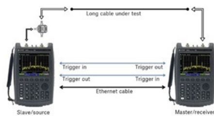
Measure long, lossy cables using ERTA set up
