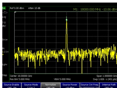
Monitor frequency spectra up to 54 GHz with FieldFox
