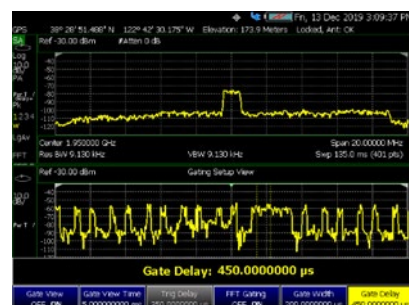
LTE FDD control channel captured with periodic frame trigger synced to GPS
