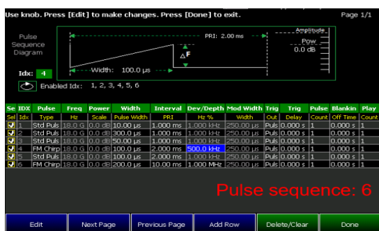
The FieldFox display showcases the user-definable pulse sequences and waveform
