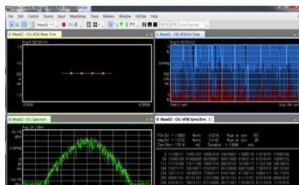
Public safety transmitting signal quality test –P25 C4FM demodulation with FieldFox
