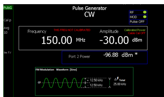
A Frequency-Modulated (FM) signal is presented with essential parameters such as carrier frequency, FM deviation, and additional details
